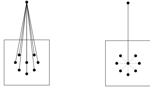
Figure 1: All nodes actually lie on top of each other and the edges pass through one portal. Figure 2: All nodes actually lie on top of each other and the dotted lines have length 0.
